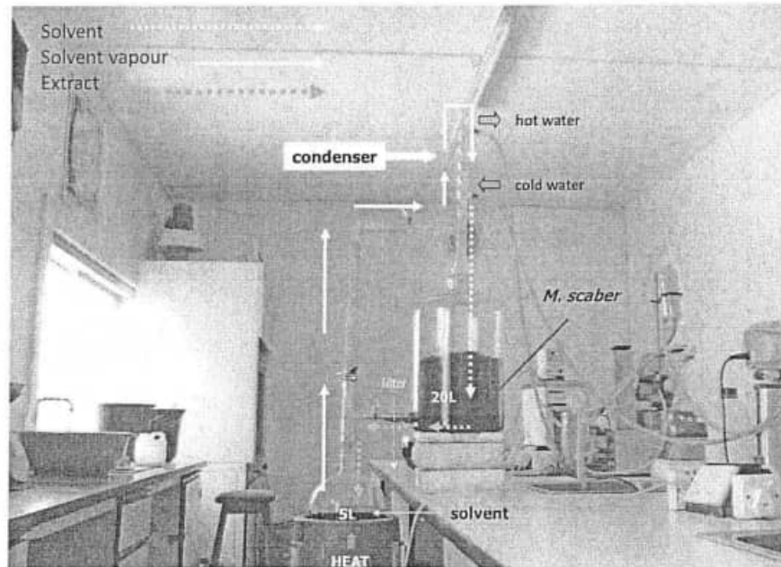
Plate 1. Setup for pilot scale preparation of M. scaber extract
